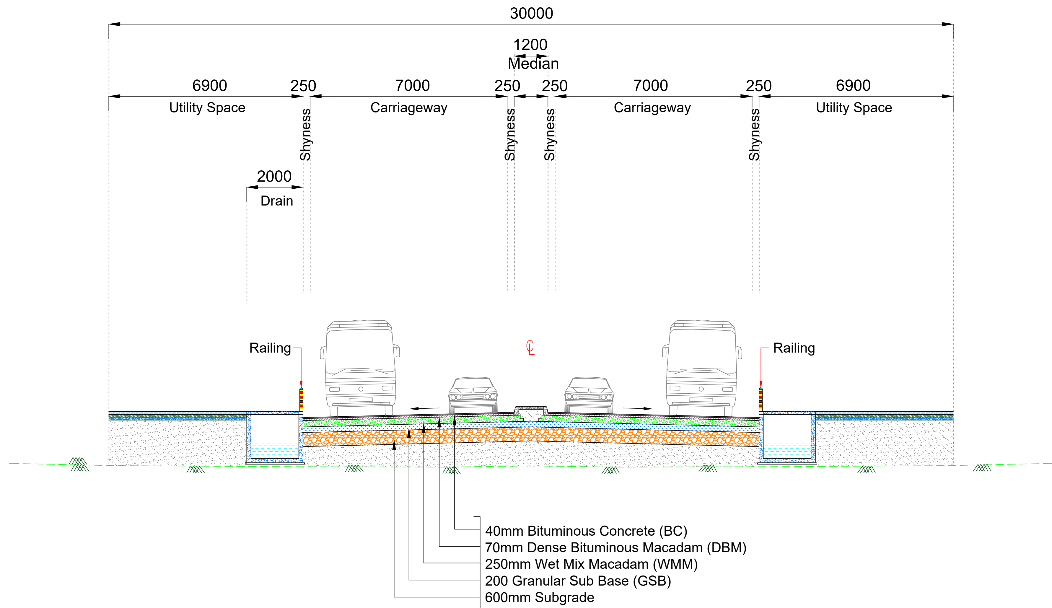
TYPICAL CROSS SECTION - TYPE S7
