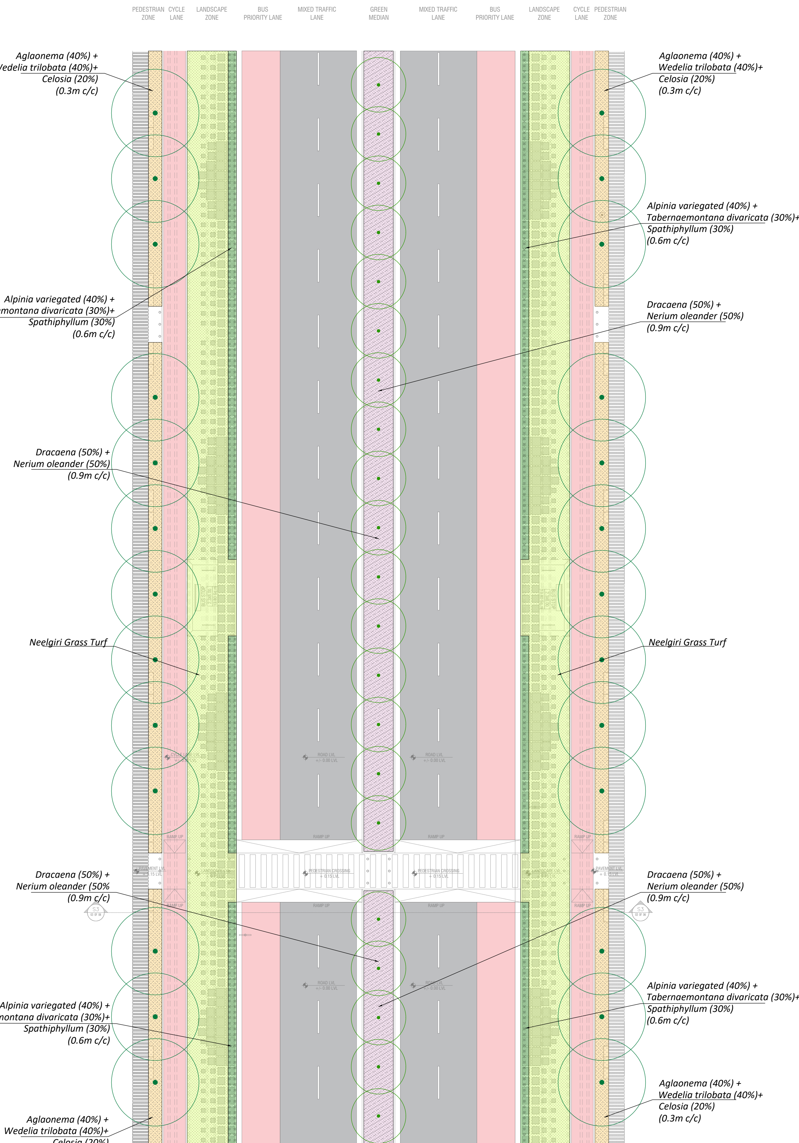
02 SUB-ARTERIAL ROAD SHRUBS AND GRASS PLANTING PLAN 02 OF 04 SCALE 1:200
