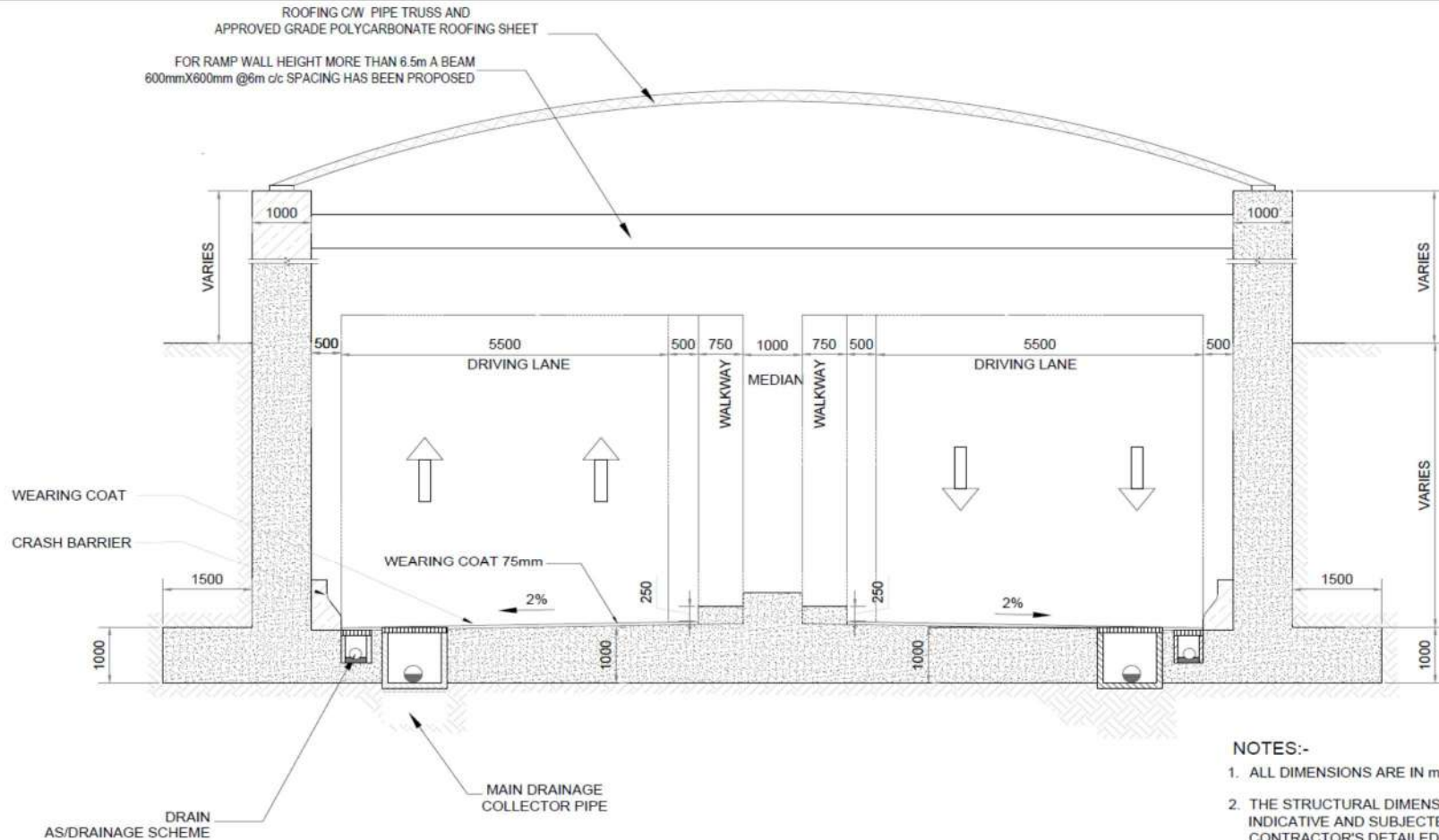
TYPICAL CROSS SECTION -11 RAMP SECTION (TYPE - RPBD3) BIDIRECTIONAL - 1.5 LANE+MEDIAN+1.5 LANE (3 LANE) REGULAR CROSS SECTION SCALE 1:50
