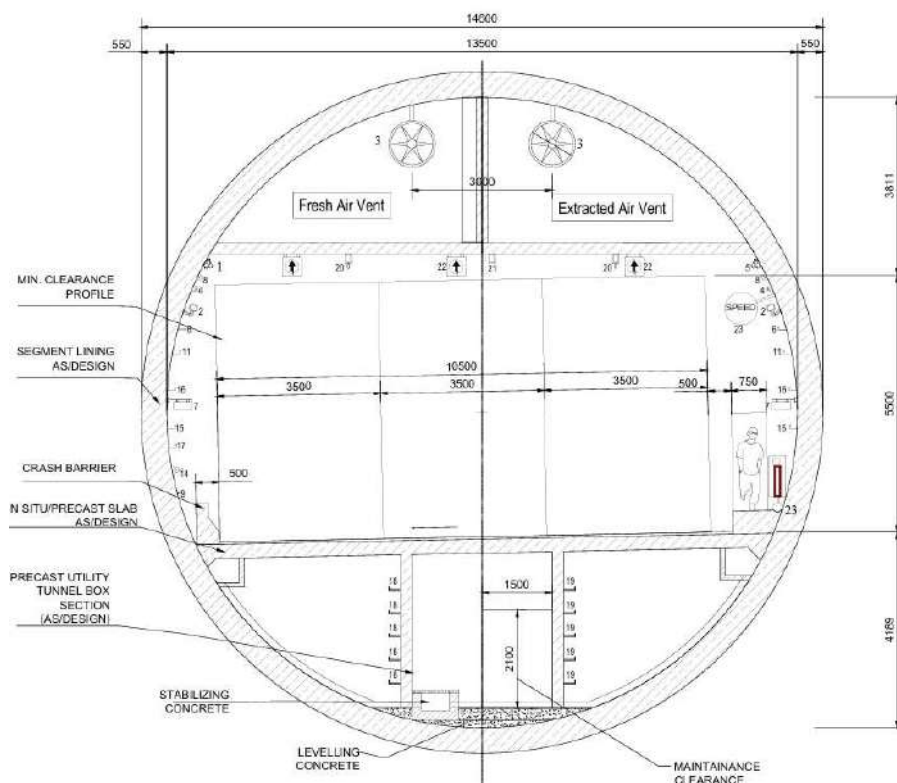
Figure 8.3: Cross section of the main tunnel showing duct and fans positioning
