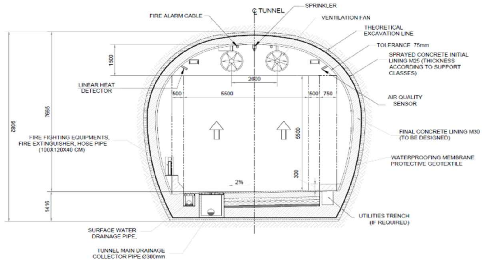
TYPICAL CROSS SECTION -15 NATM TUNNEL (INTERMEDIATE LANE) SCALE 1:50
