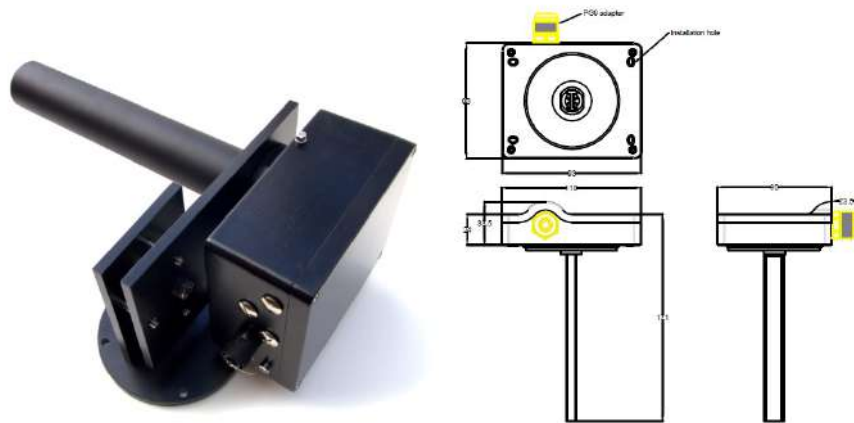
Figure 8.1: Air monitoring system
