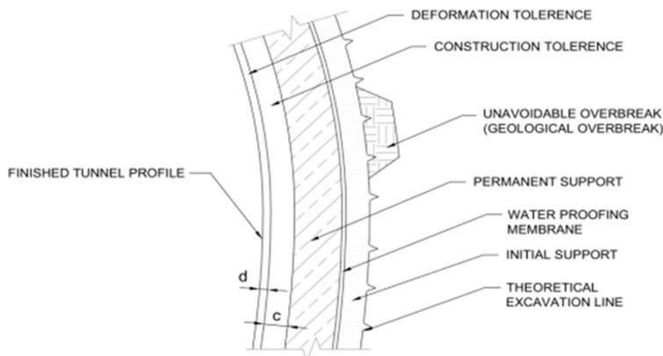
Figure 4.1 - Definition of Deformation and Construction Tolerances
