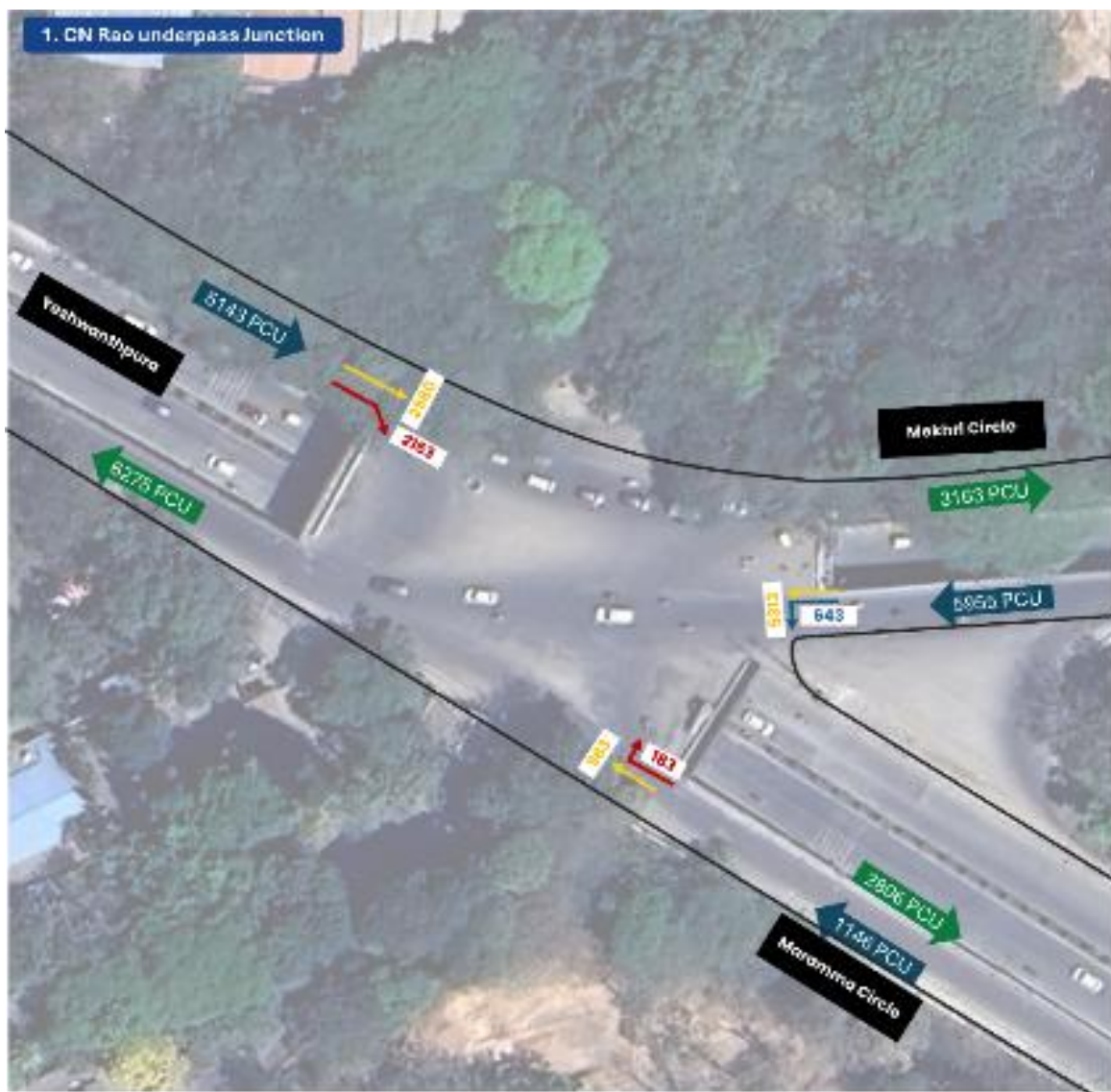
Figure 95: TMC at CN Rao Underpass Junction
