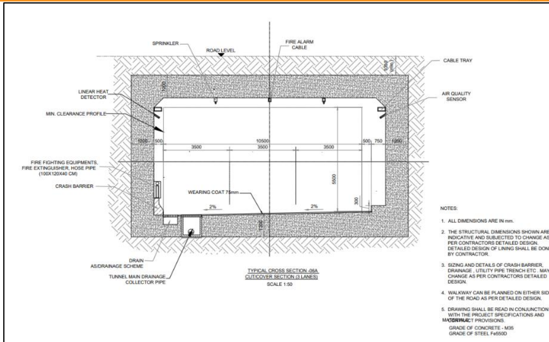
Figure 123: TCS-6A, 3 Cut and Cover Section
