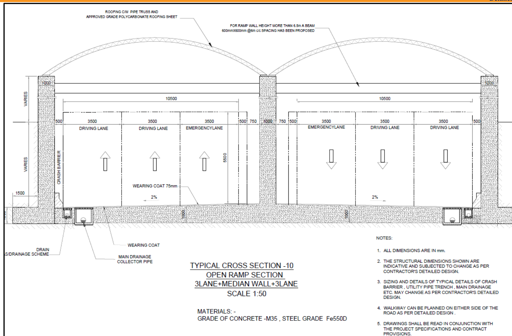
Figure 127: TCS-10, 3+3 Lane Open Cut Section
