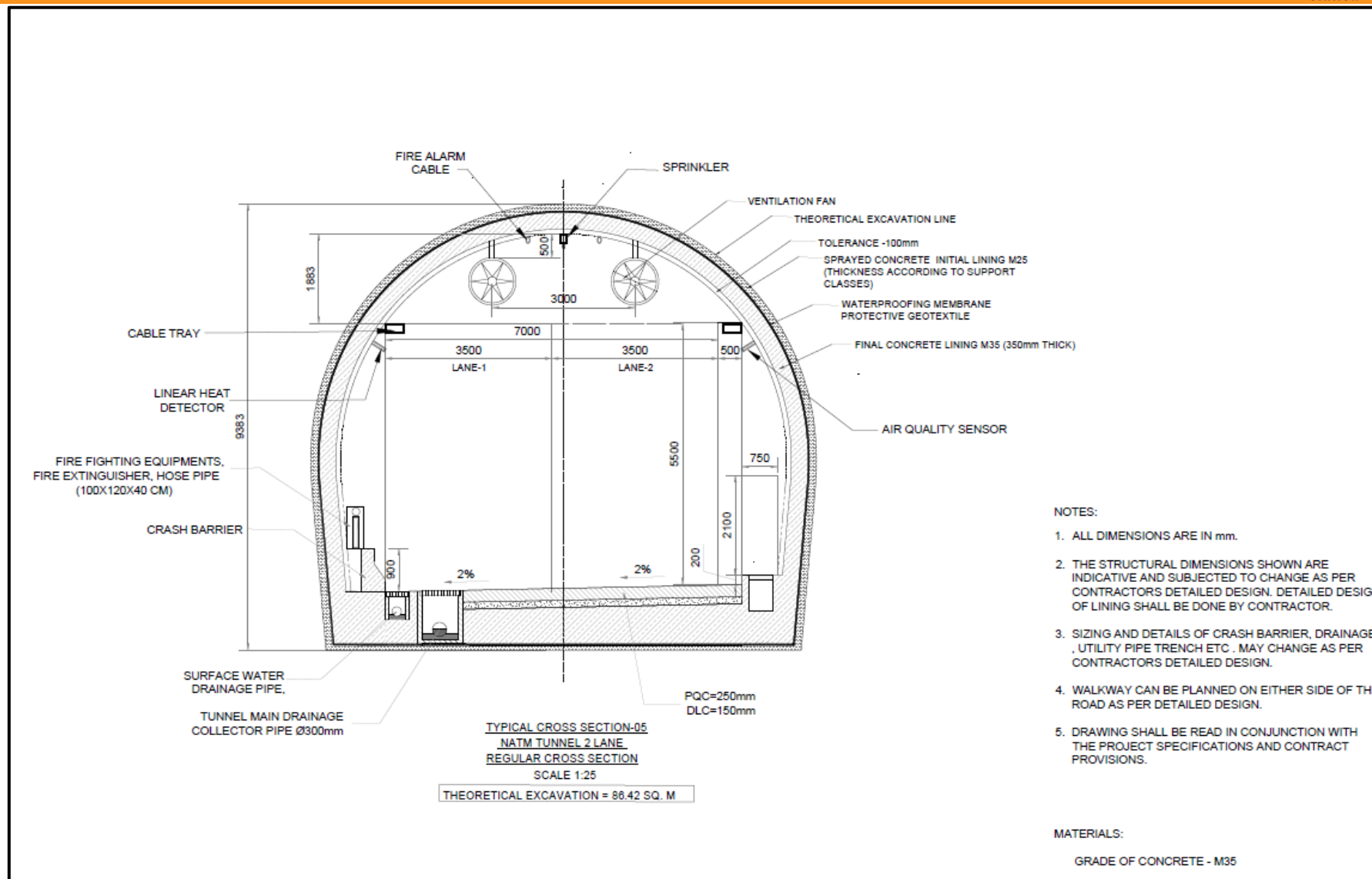
Figure 121: TCS-5, 2 Lane NATM Section
