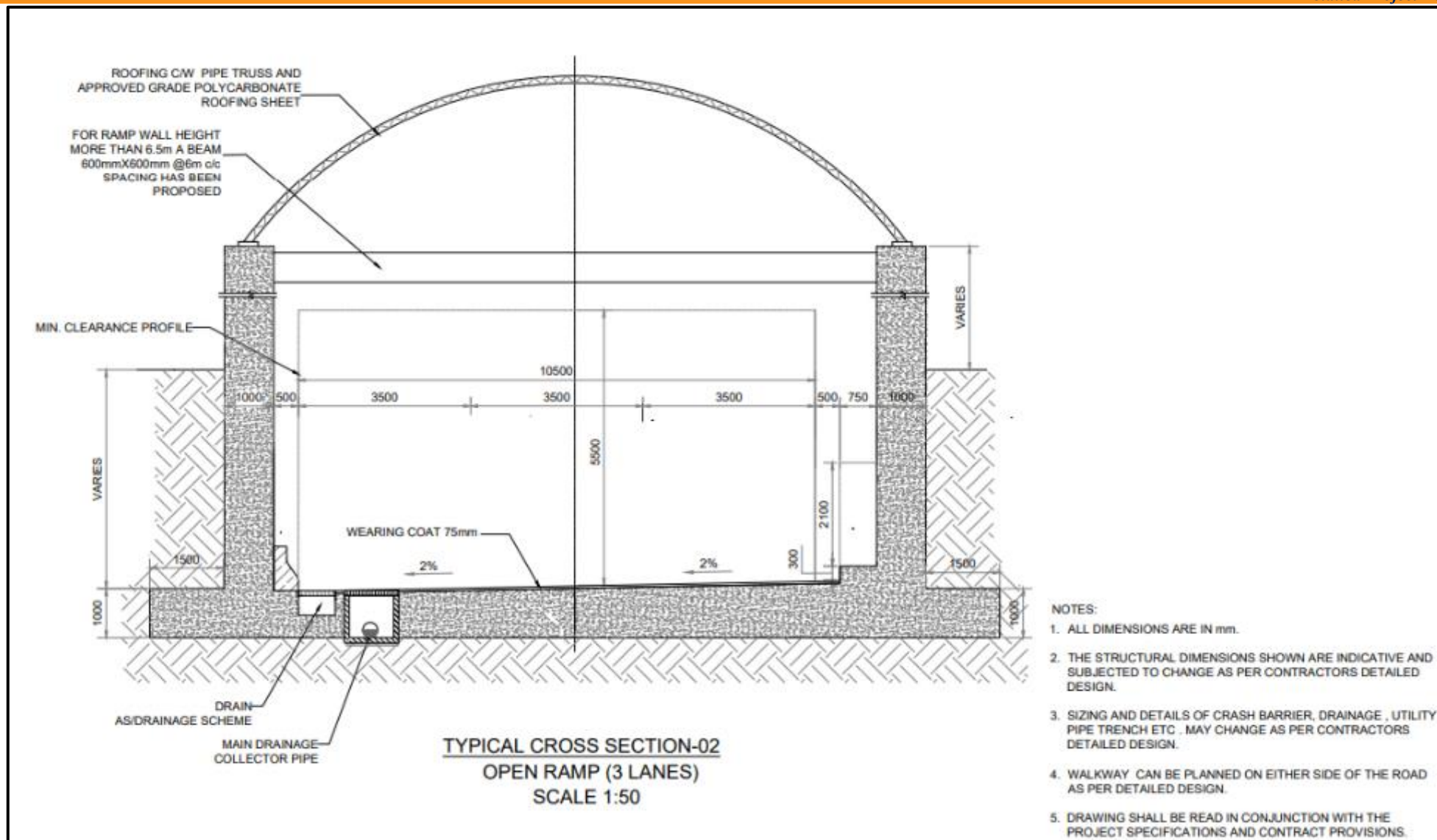
Figure 117: TCS-2, 3 lane Open Cut Section
