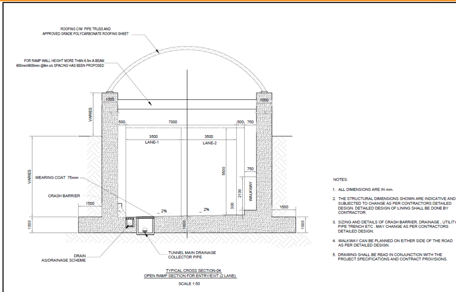
Figure 120: TCS-4, 2 lane Open Cut Section
