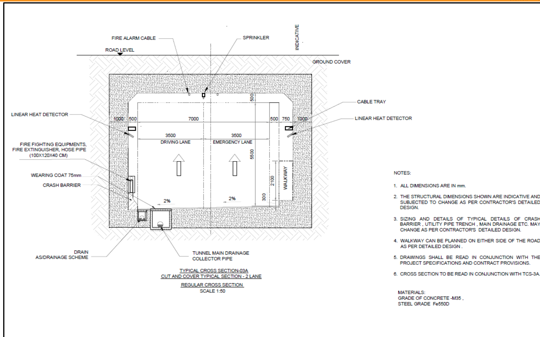
Figure 119: TCS-03A, 2 lanes Cut and Cover
