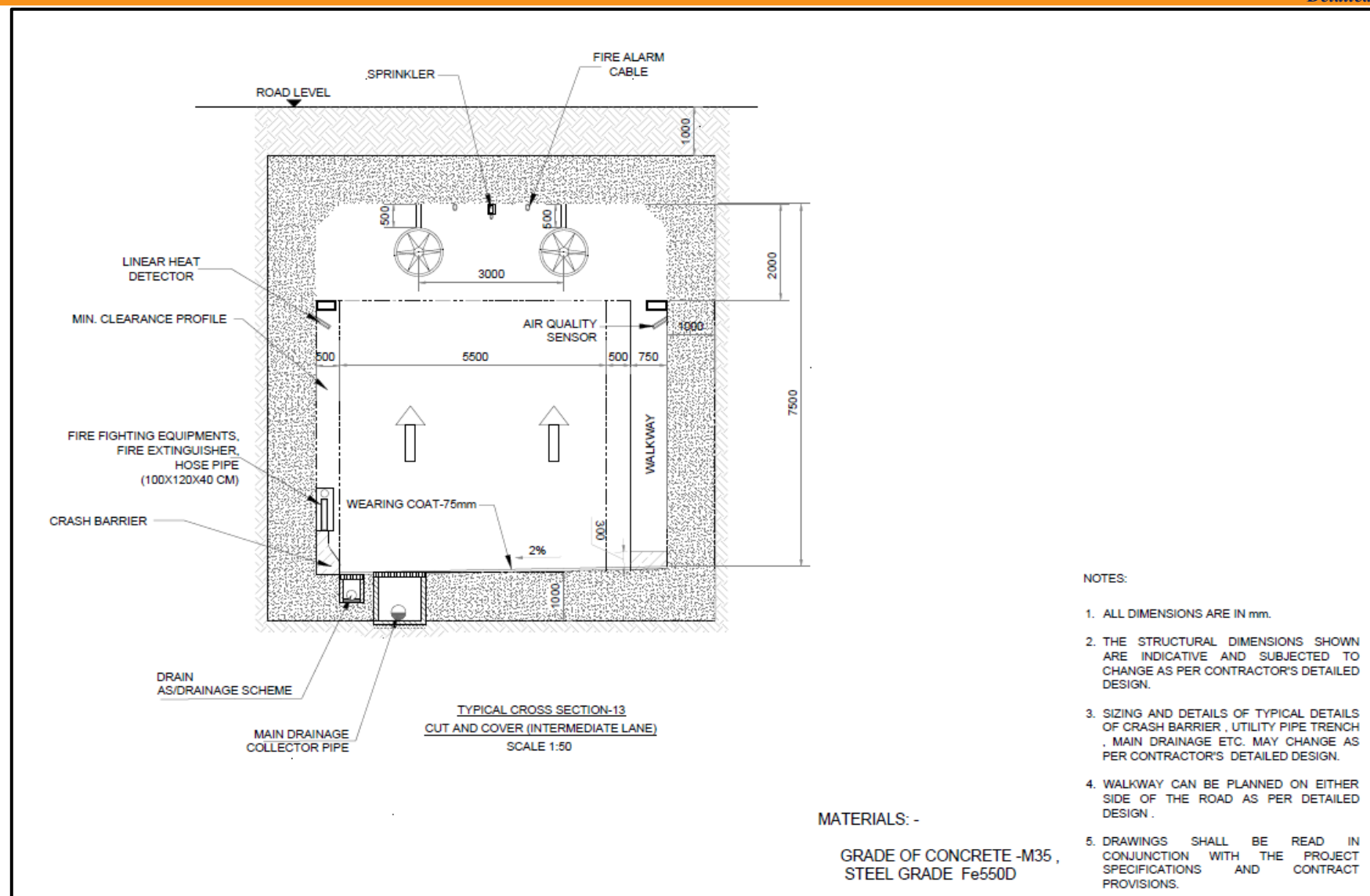
Figure 131: TCS-13, Intermediate Lane Cut and Cover Section
