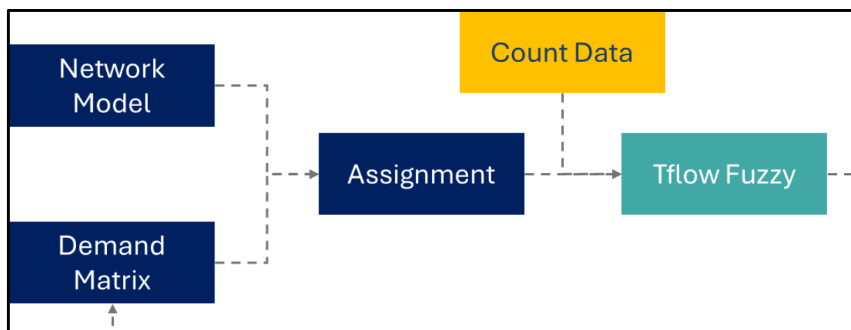
Figure 55: Fuzzy Procedure
