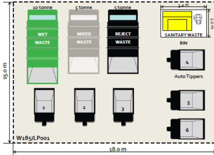
Figure 09: Normative standards for a typical lorry point
