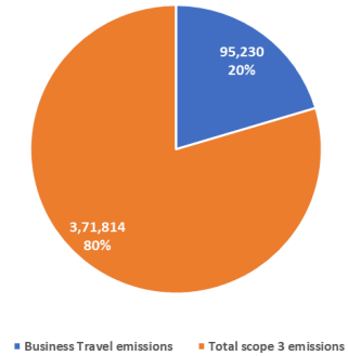
Graph 38: Contribution of Business Travel Emissions to Scope 3 emissions in FY 2022-23 - Cognizant
