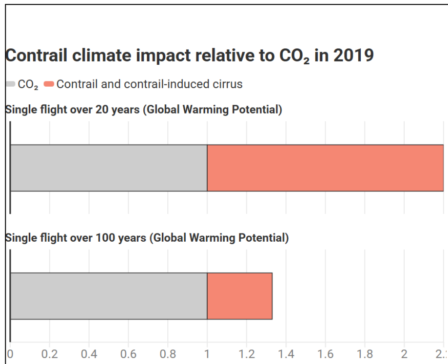
Fig. 2: The Global Warming Potential of Contrails (Source: Transport and Environment )
