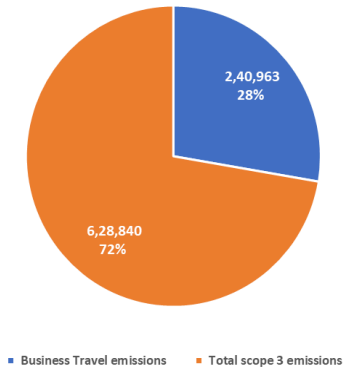
Graph 32: Contribution of Business Travel Emissions to total Emissions in FY 2023-24 – Accenture
