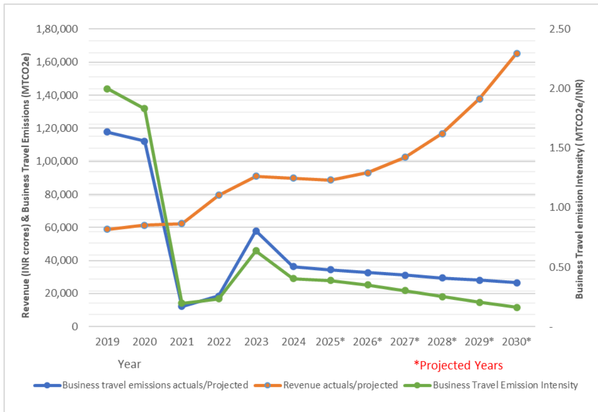
Graph 12: Business Travel Emissions, Revenue, and Business Travel Emission Intensity - Performance Actuals and Projected
