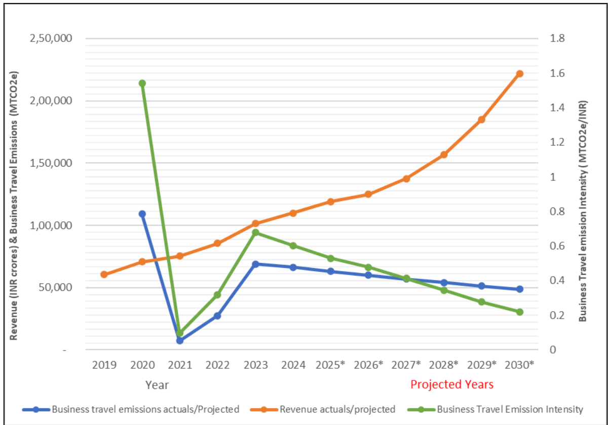
Graph 18: Business Travel Emissions, Revenue and Business Travel Emission Intensity - Performance Actuals and Projected.
