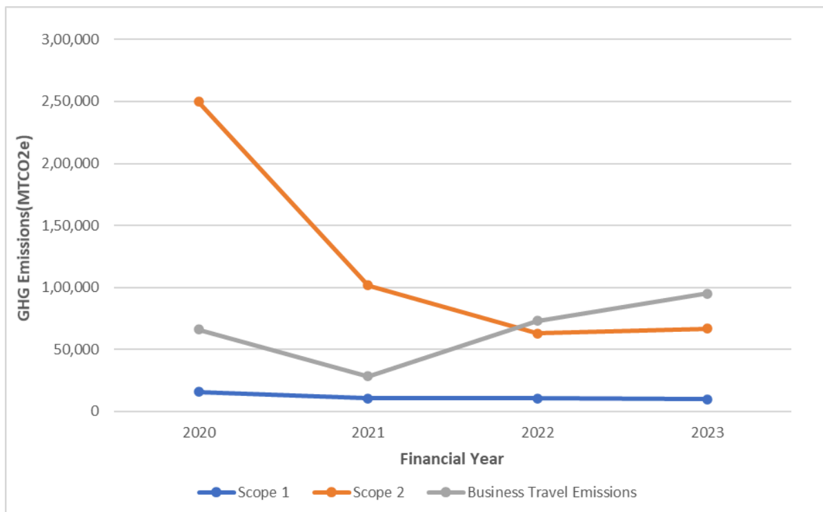
Graph 39: Business Travel Emissions Performance Against Scope 1 and 2 Emission Performance
