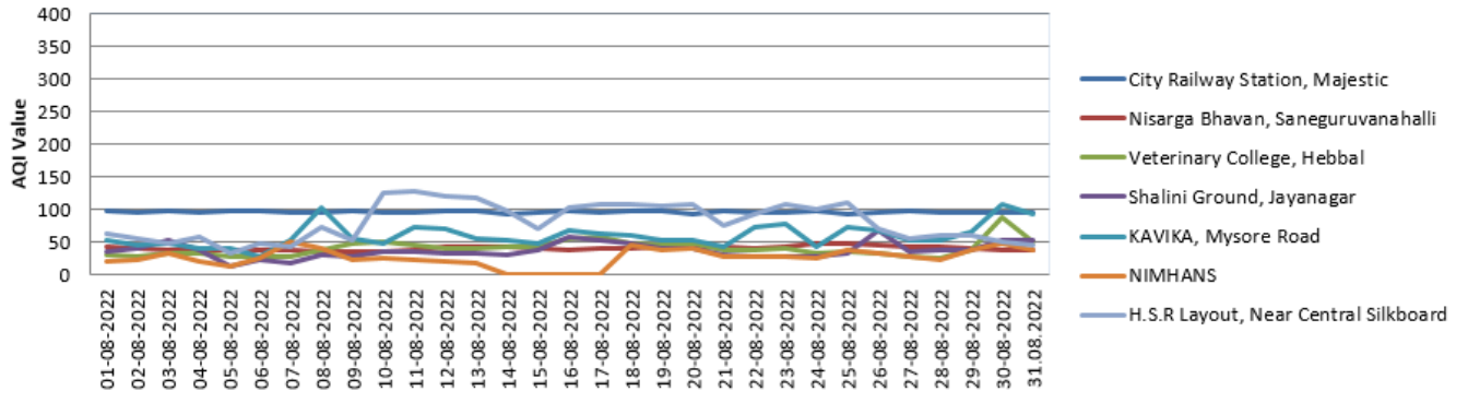
AAI trend in CAAQM Station, August-2022
