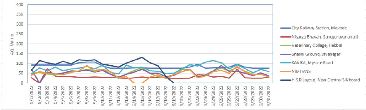
AAQI Trend in CAAQMs Station, May-2022
