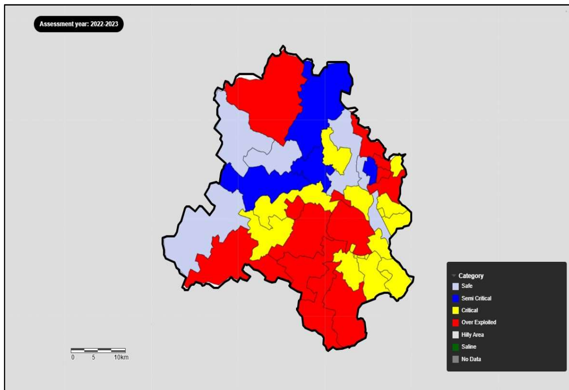
Categorization Map of GWRA 2023 – Delhi
