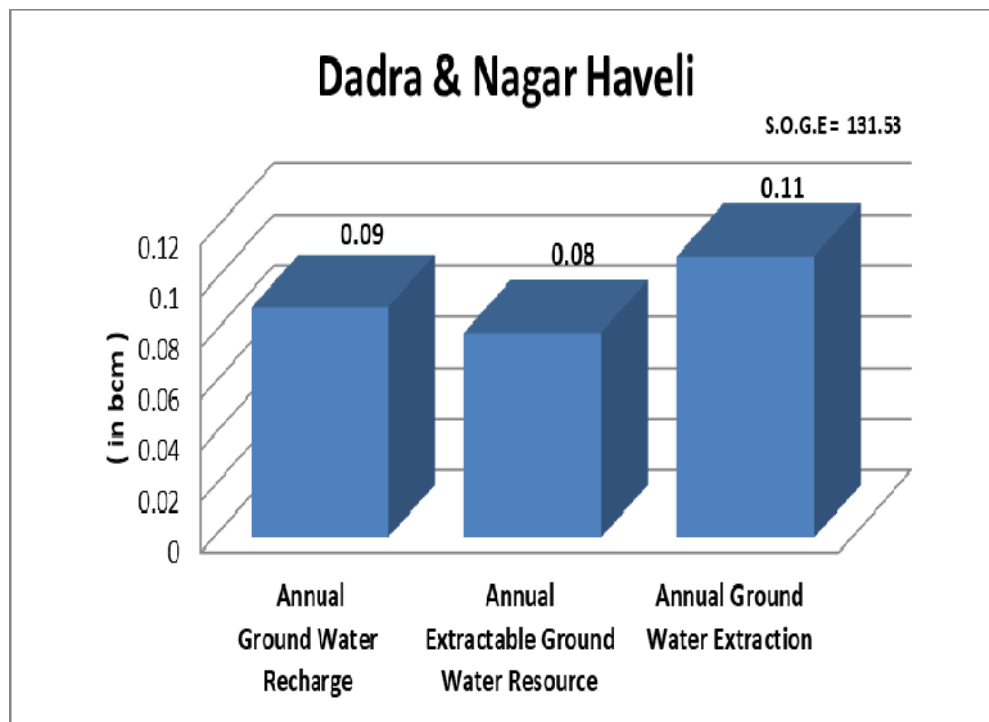
Dynamic Ground water Recourses Scenario 2023 – Dadra and Nagar Haveli
