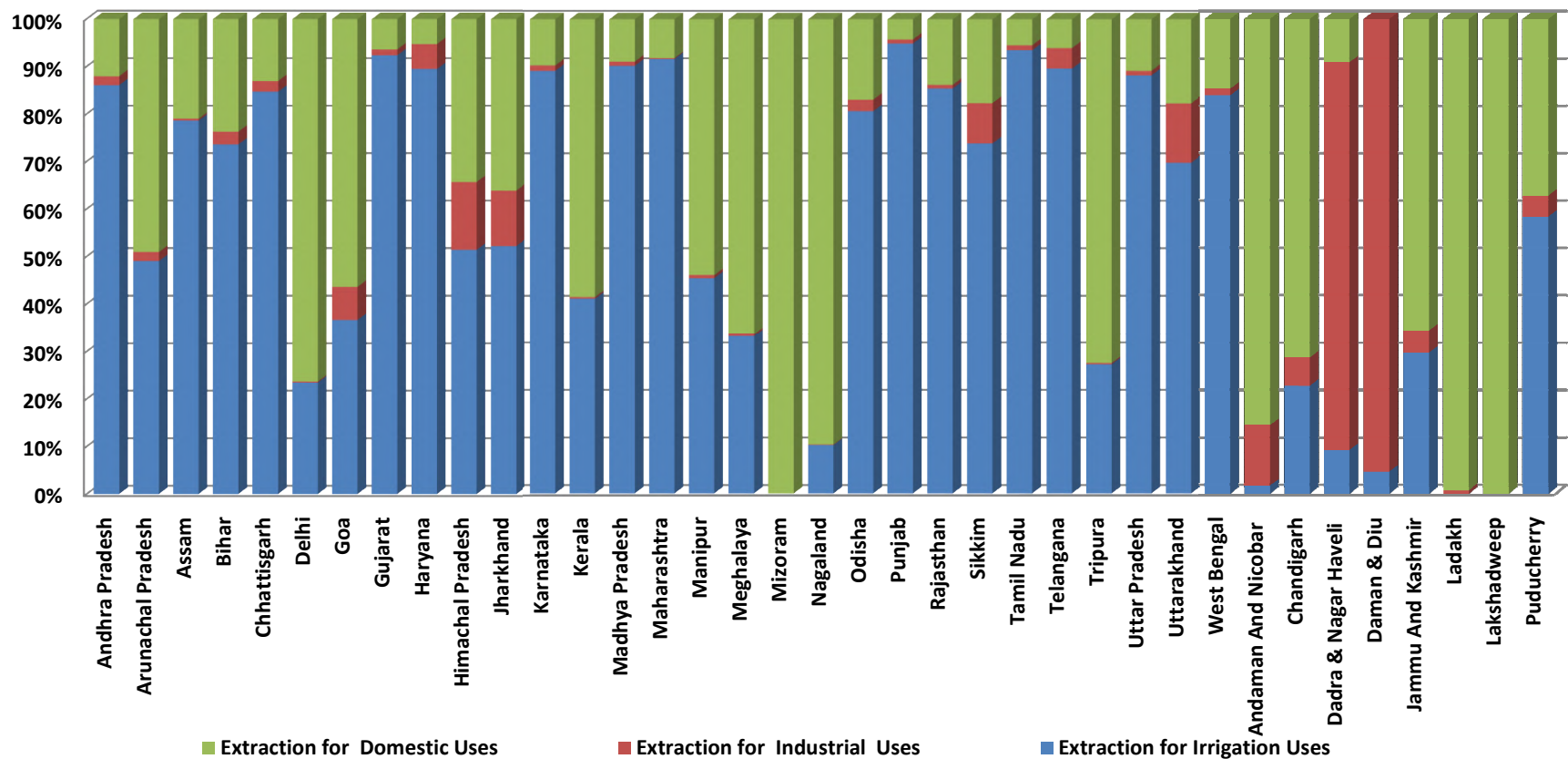
Fig-6.4: State wise % of Groundwater extraction for Irrigation vs. Industrial and Dometic Purposes
