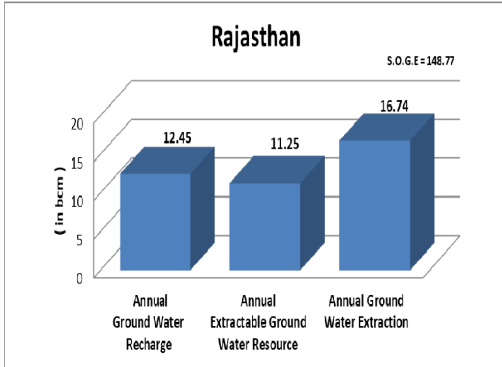
Dynamic Ground water Recourses Scenario 2023 – Rajasthan
