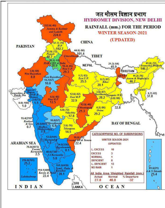
Figure-3.2 : Winter Rainfall Map
