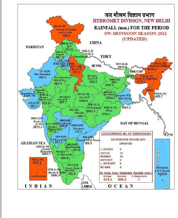
Figure-3.4 : SW Monsoon Rainfall Map
