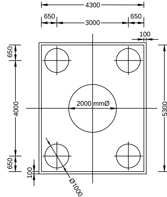
Pile Cap for 8.5m Width of Carriageway
