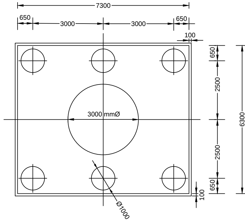
Pile Cap for 15/17m Width of Carriageway
